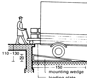
6 Permanent or portable dock leveller
